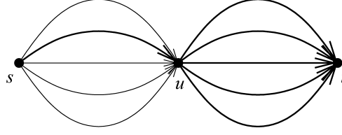
FIG. 3. The graph G for the maximum flow game.
