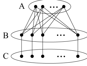
FIG. 1. Vertex cover sample distribution.
